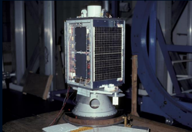
UoSat-OSCAR 9 UoSat OSCAR 11 – Beacons on 2.4 GHz and 10.5 GHz
